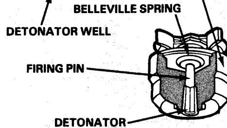
ALUMINUM FUZE CASE
